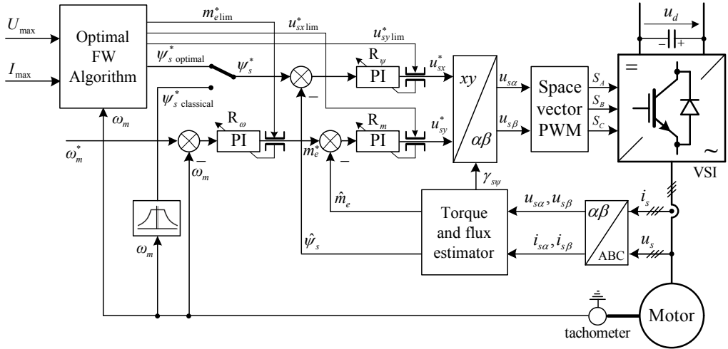
Fig. 6. Block diagram of the SVM-DTC
