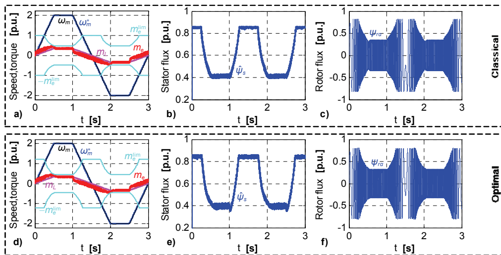
Fig. 9. Start up, steady state at \omega_m = 2.0 [p.u.] speed and braking cycle in both directions for two FW methods: classical (a, b, c) and proposed (d, e, f); (a, d) reference and motor speeds, load, limit and motor torques, (b, e) estimated stator flux, (c, f) rotor flux
