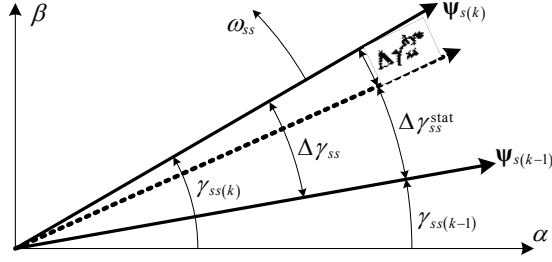
Fig. 3. Stator flux vector position components
