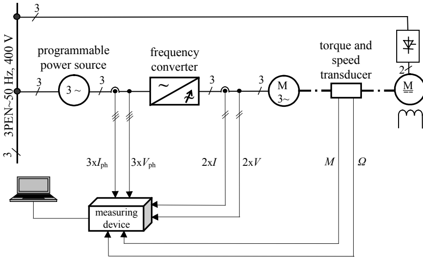
Fig. 1. Block diagram of the tested drive
