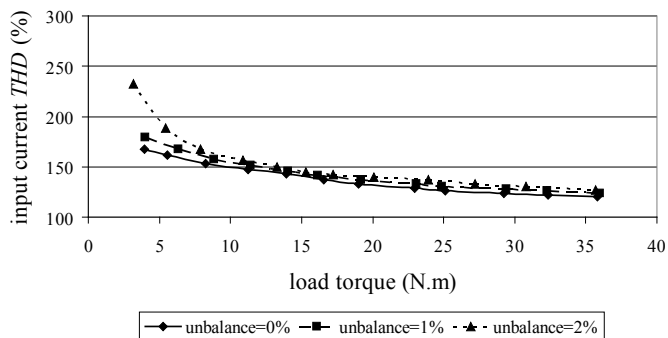
Fig. 7. Total input current harmonic distortion THD_I versus load under adjusted levels of voltage unbalance ( f = 50 Hz, THD_V = 0.5\% )
